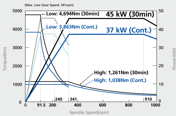
Hi-TECH 850BB/Hi-TECH 850BB+ (Turnmill)
